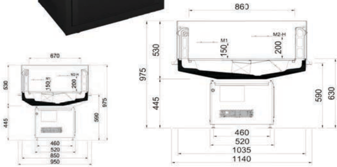
LS 670, LS 860 Low-Set (width 1250mm)
