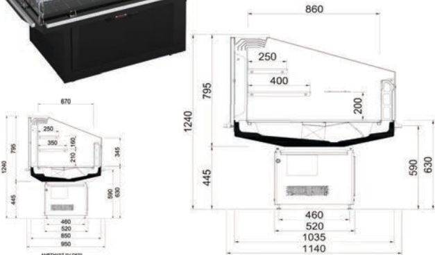
SV 670, SV 860 Semi-Vertical (width 1250mm)
